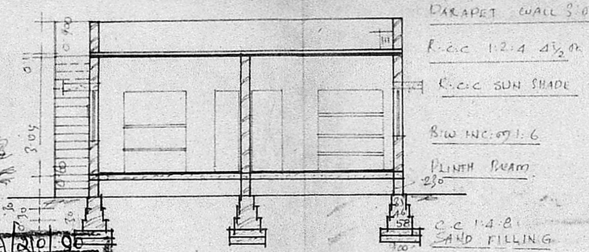
SECTION ON 1B
